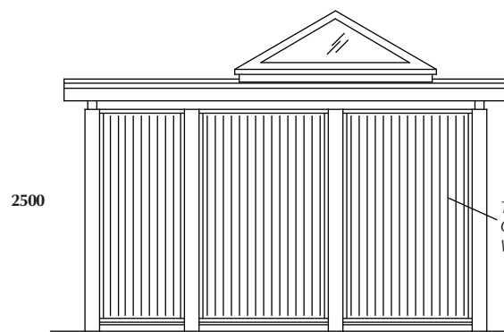
BACK ELEVATION
